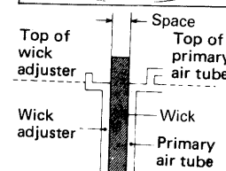
Wick Adjuster (Cutaway view)
