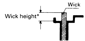
Wick Adjuster (Cutaway view)
